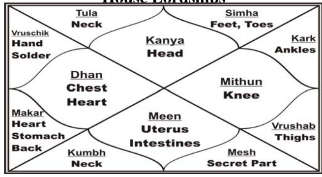
Rasi - General
