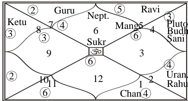
Ravi
