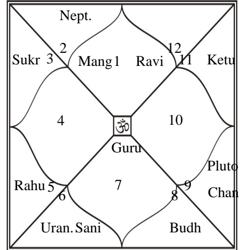
Navamsa Chart
