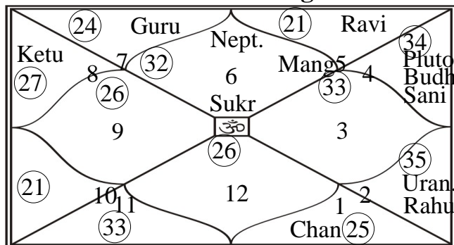
Sarvashtakvarga
