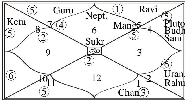
Chan
