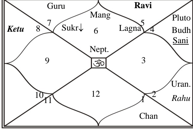
Chalit Chart
