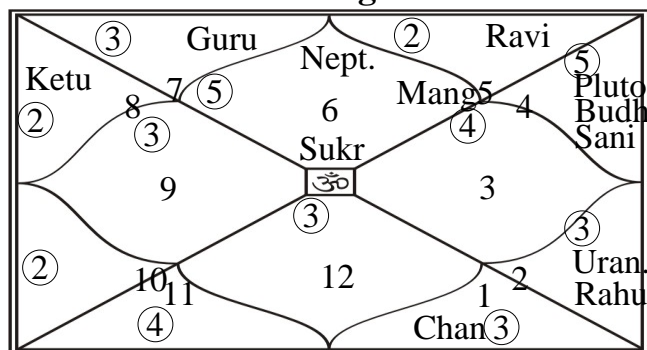
Guru
