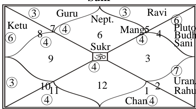
Sarvashtakvarga
